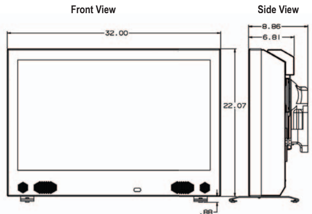
TV Dimensions are: 32.00 in. W x 22.07 in. H x 6.81 in. D Height dimension with table stand is 22.95 in. TV with optional wall mount measures 8.86 in. when folded flush against the wall.
